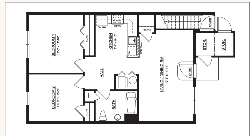
2 Bedroom First Floor (Continued on back)
