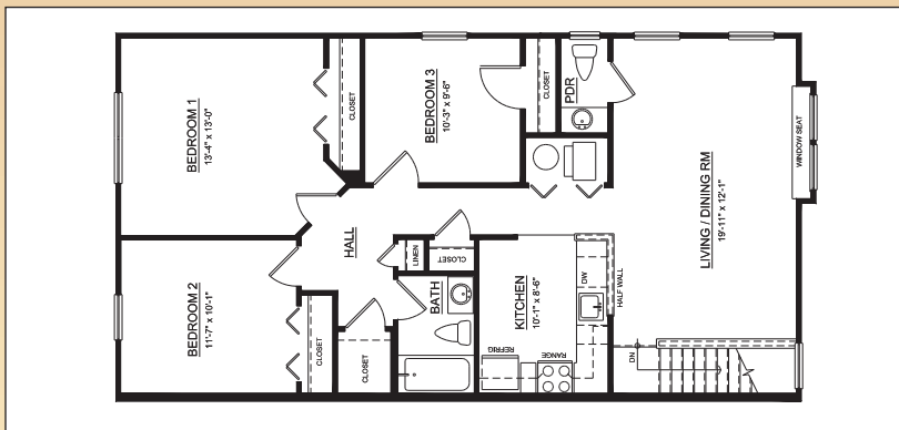
3 Bedroom Second Floor
