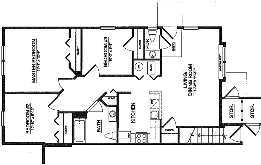
UNIT 'C' FIRST FLOOR PLAN (HANDICAP ADAPTABLE UNIT) (THREE BEDROOM)
