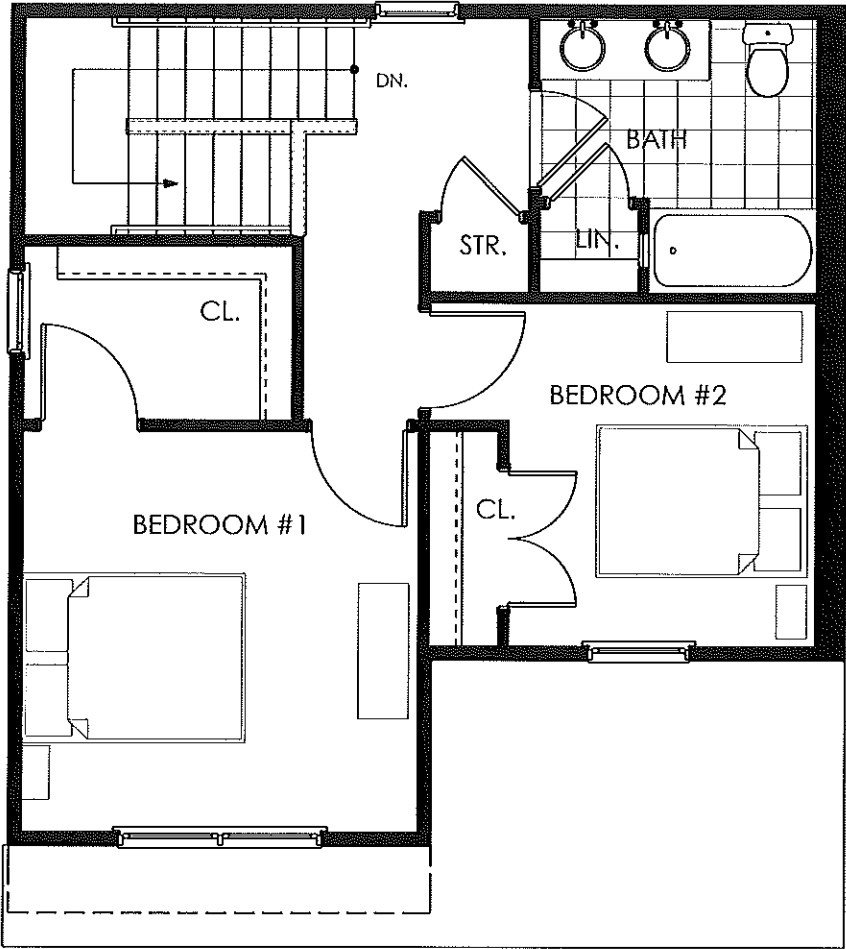
2 BEDROOM UNIT SECOND FLOOR
