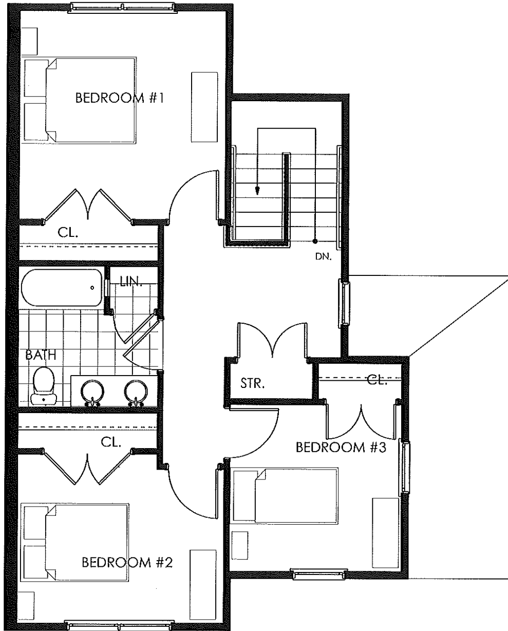
3 BEDROOM UNIT SECOND FLOOR
