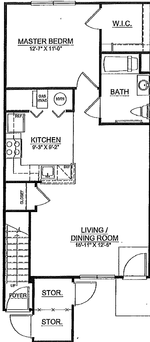
FIRST FLOOR PLAN UNIT 'A'
