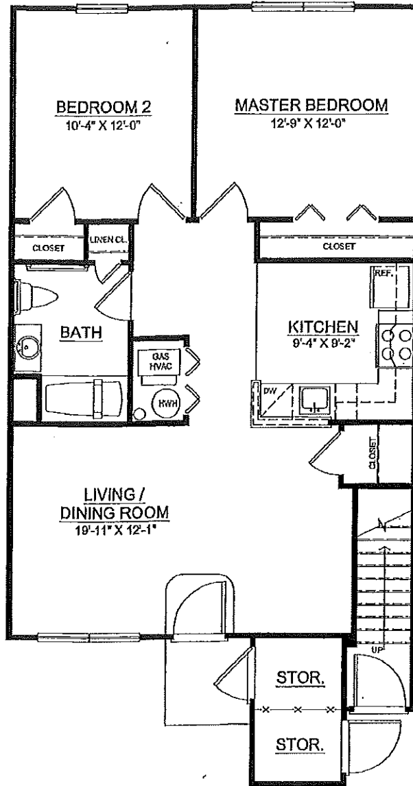
FIRST FLOOR PLAN UNIT 'B'
