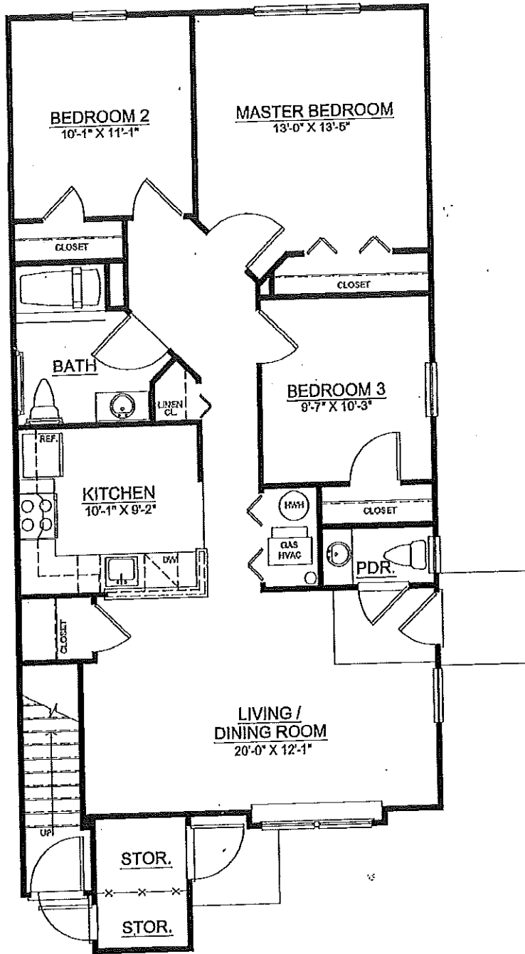
FIRST FLOOR PLAN UNIT 'C'
