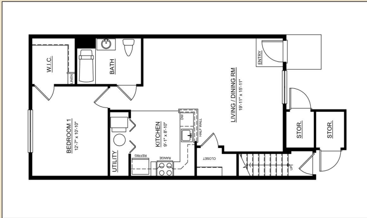
First Floor Plan (One Bedroom)
